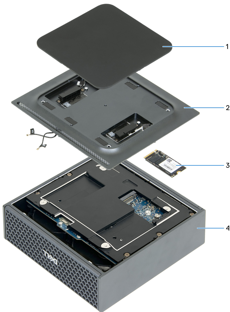
Figure 14. Major Components of Dell Pro Max with GB10
